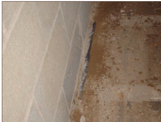
Figure A4.64 Insufficient length of gas membrane protruding through wall to overlap with gas membrane within building (courtesy Card Geotechnics Limited)
